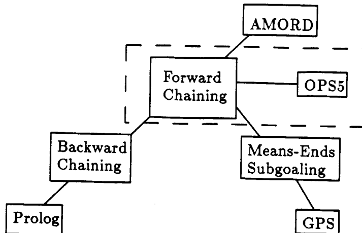
Figure 6-1: Rule System Design Space.
