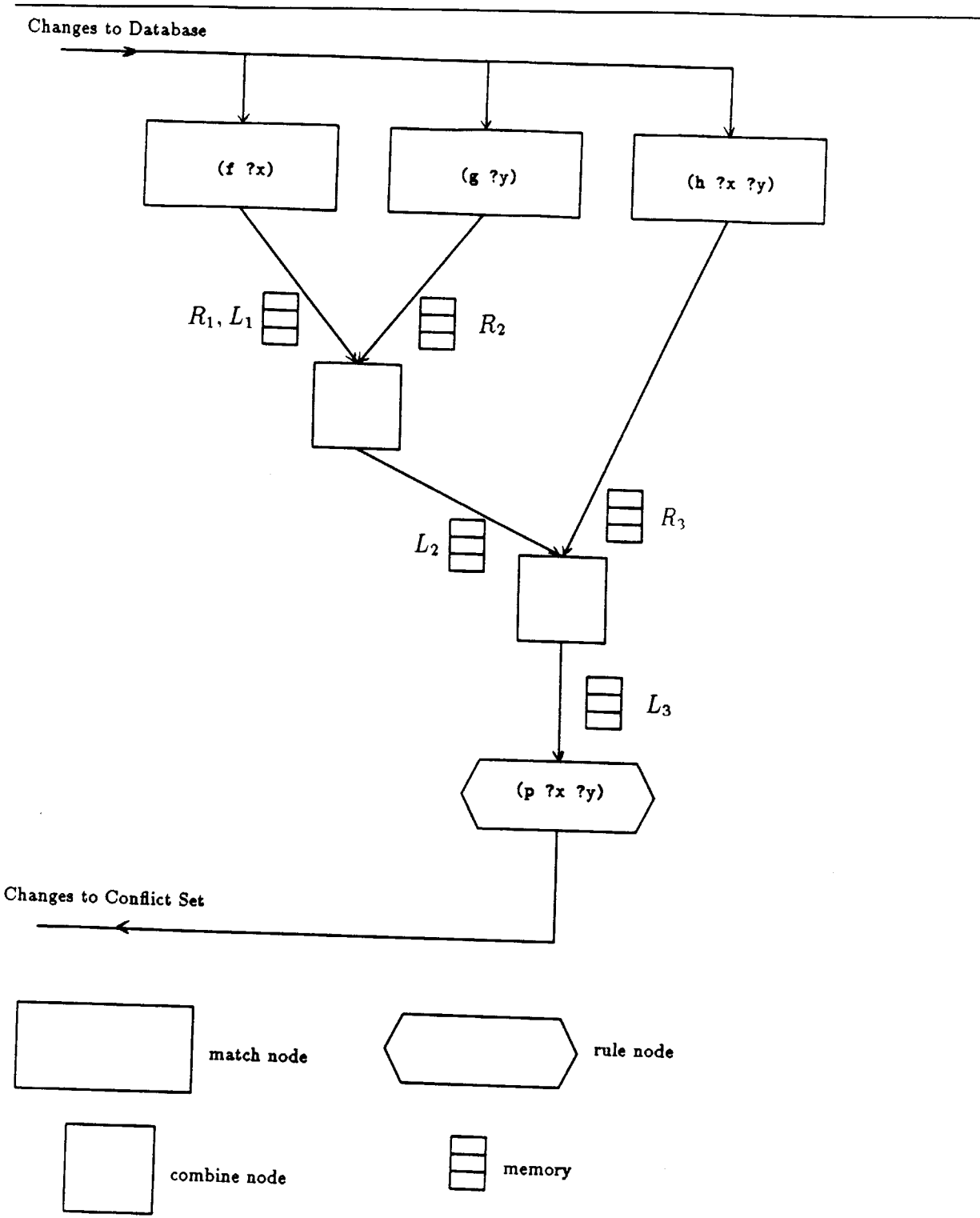
Figure 4-2: Correspondence between Match-Rule and the Rete Network.
