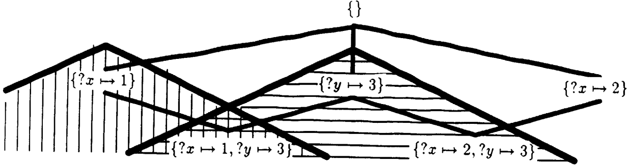
Figure 3-4: Intersection of two Ideals in the Substitution Semi-Lattice.
